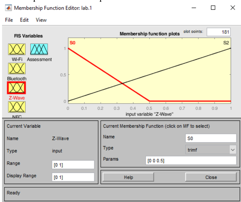
Рис. 2 Membership Function Editor.
